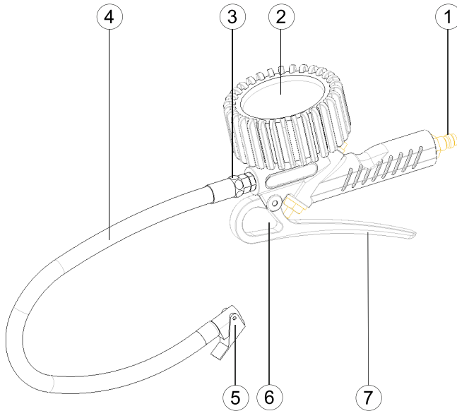
Image 1. Assemblies
